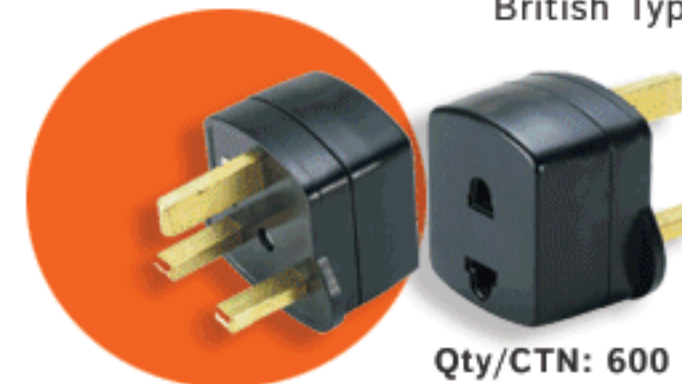
British Type Adapter Plug-3 Square Metal pins
